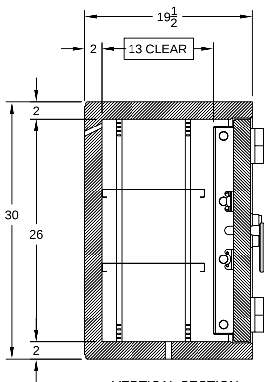
VERTICAL SECTION (CLOSED DOOR)
