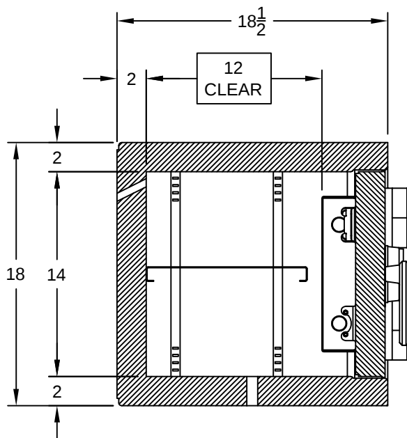
VERTICAL SECTION (CLOSED DOOR)
