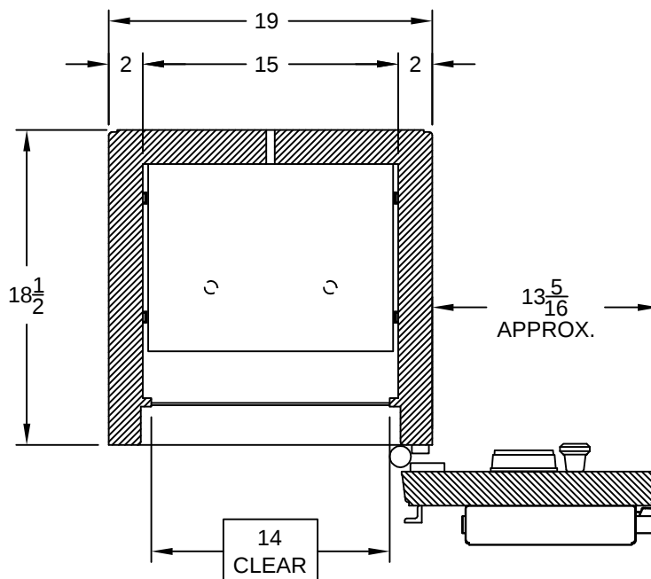
HORIZONTAL SECTION (DOOR OPENED AT 180°)
