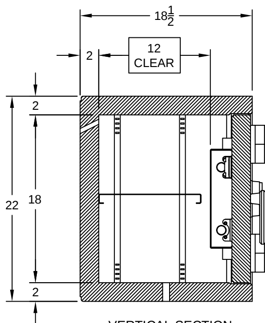
VERTICAL SECTION (CLOSED DOOR)
