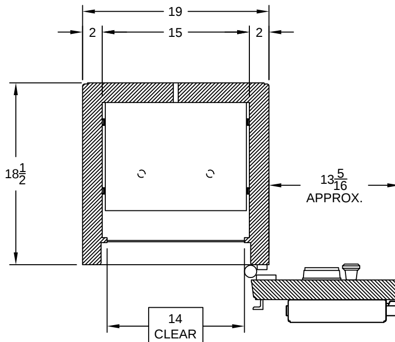
HORIZONTAL SECTION (DOOR OPENED AT 180°)
