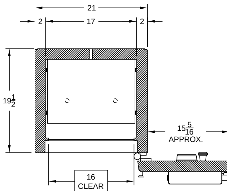
HORIZONTAL SECTION (DOOR OPENED AT 180°)
