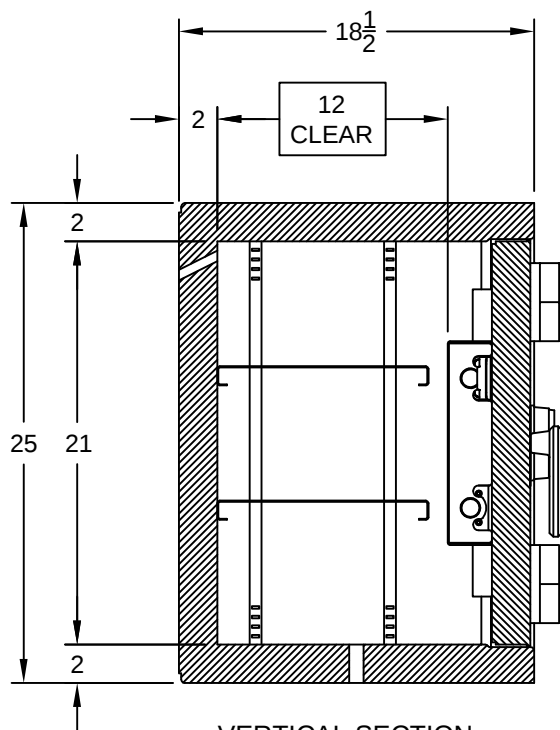
VERTICAL SECTION (CLOSED DOOR)
