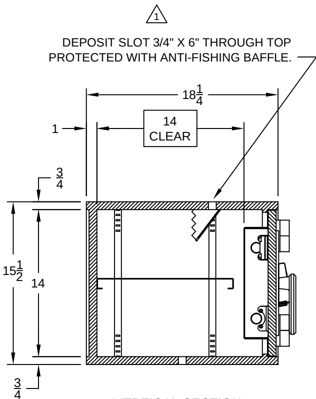
VERTICAL SECTION (CLOSED DOOR)
