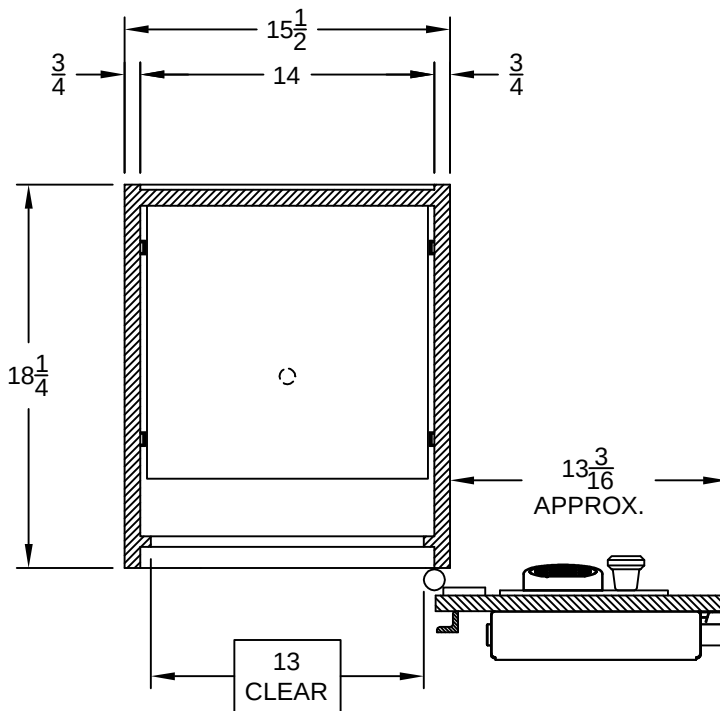
HORIZONTAL SECTION (DOOR OPENED AT 180°)
