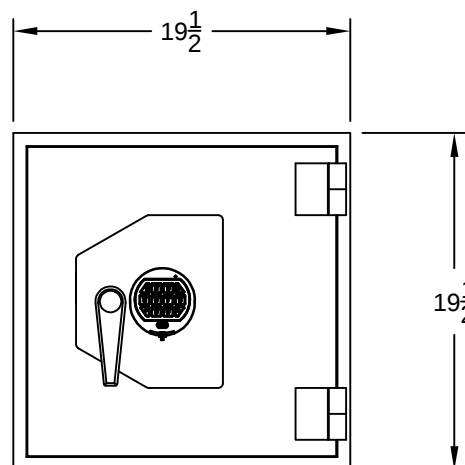
FRONT VIEW (CLOSED DOOR)
