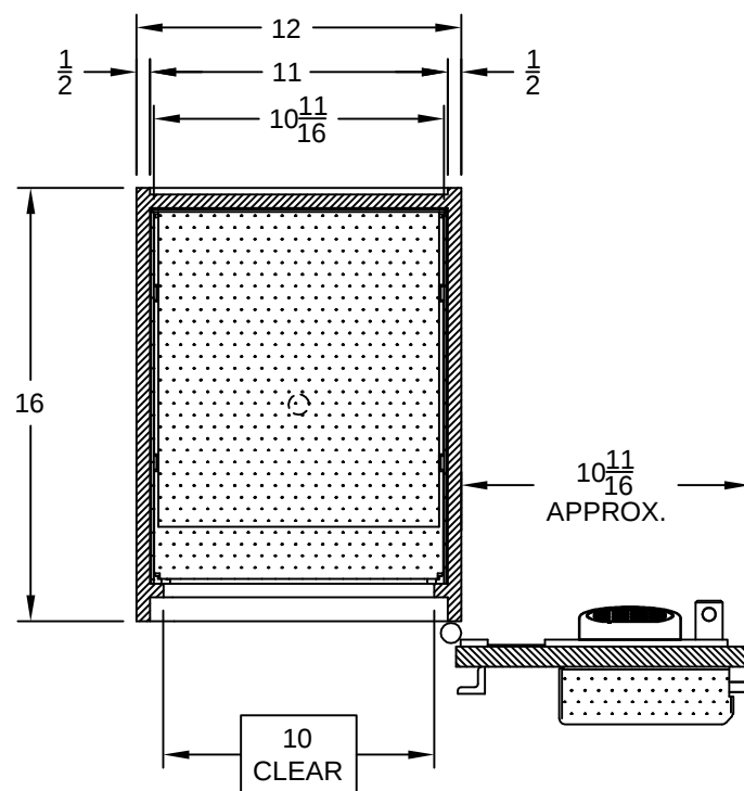
HORIZONTAL SECTION (DOOR OPENED AT 180°)
