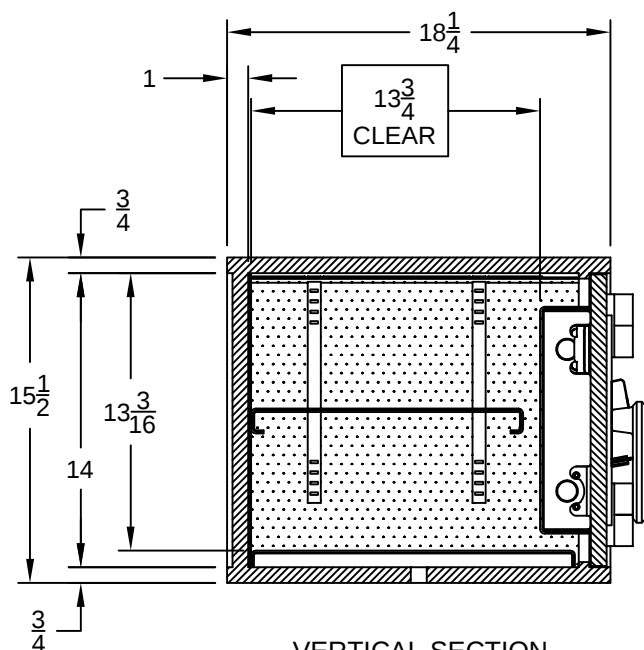
VERTICAL SECTION (CLOSED DOOR)
