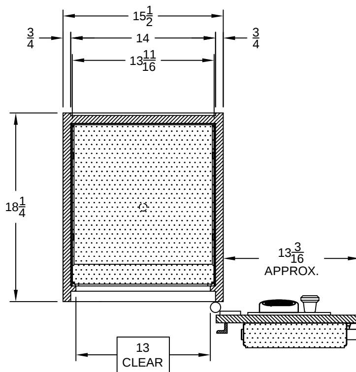
HORIZONTAL SECTION (DOOR OPENED AT 180°)
