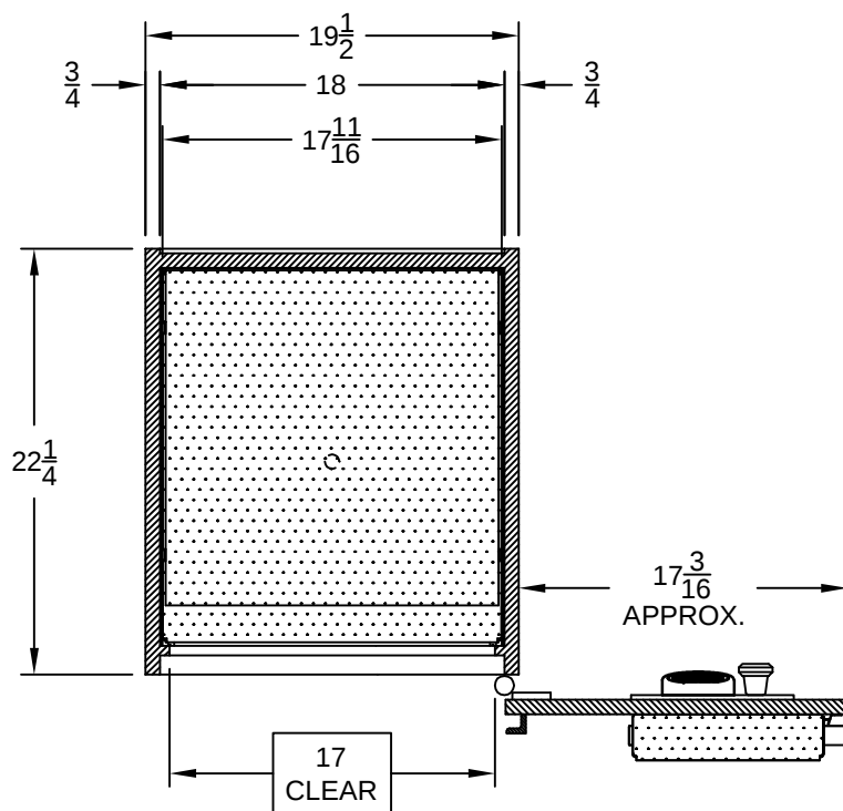
HORIZONTAL SECTION (DOOR OPENED AT 180°)
