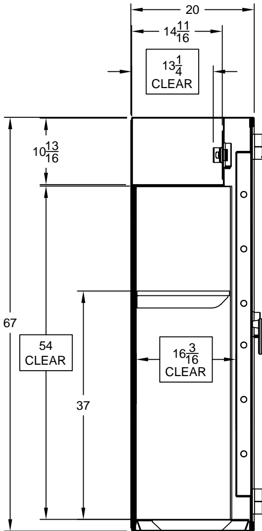
VERTICAL SECTION (CLOSED DOOR)
