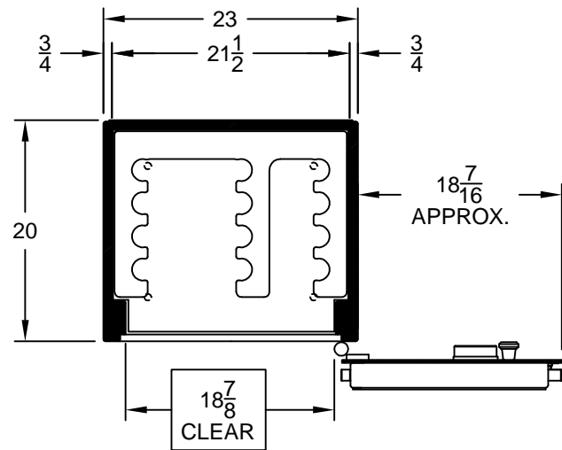
HORIZONTAL SECTION (DOOR OPENED AT 180°)
