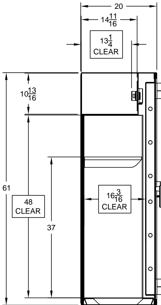
VERTICAL SECTION (CLOSED DOOR)
